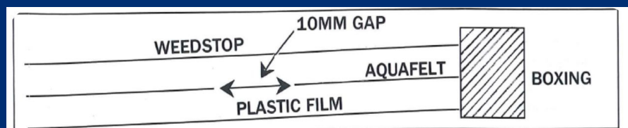
DIAGRAM #1: Capillary Watering on sloping sites. Fall should not be more than 50mm/1m.
